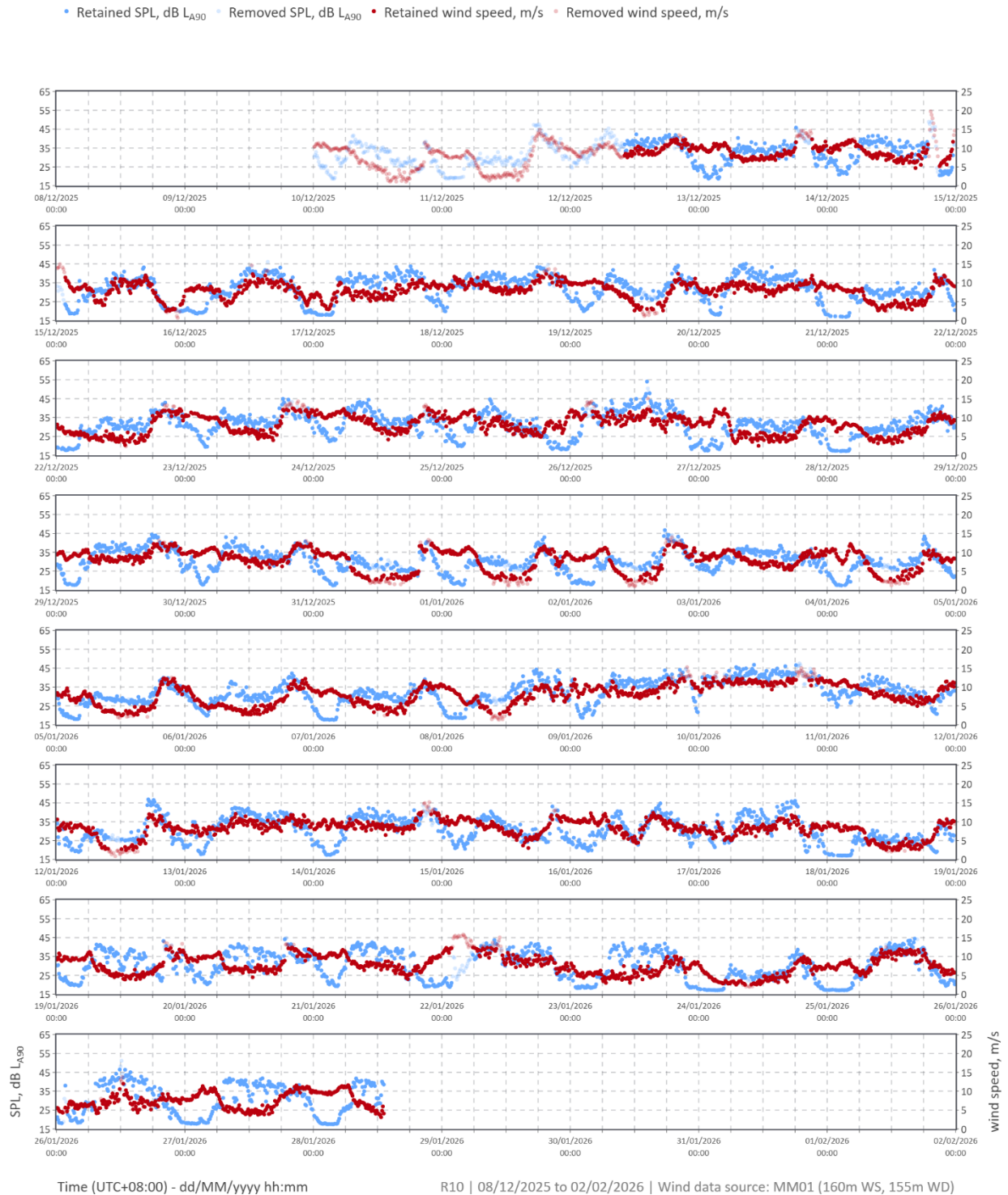
Figure 15: Location R10 background noise level and wind speed time history
