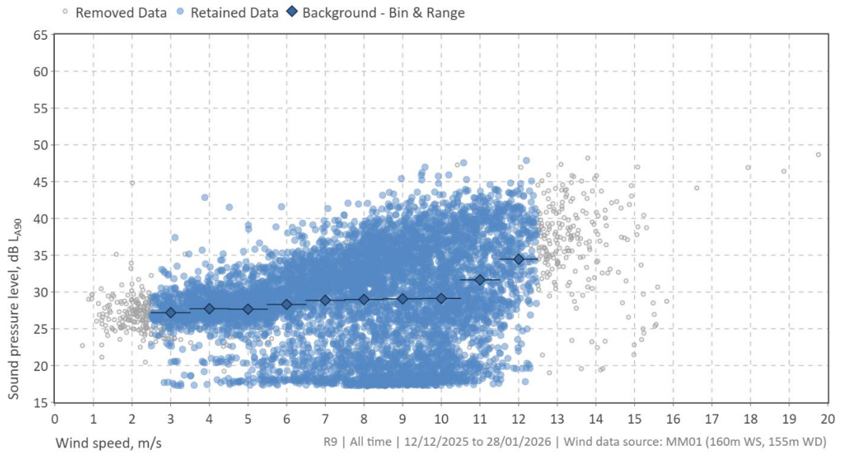
Figure 13: Location R9 derived background noise levels – 1900–0700 hrs (DWER 10 th percentile analysis)
