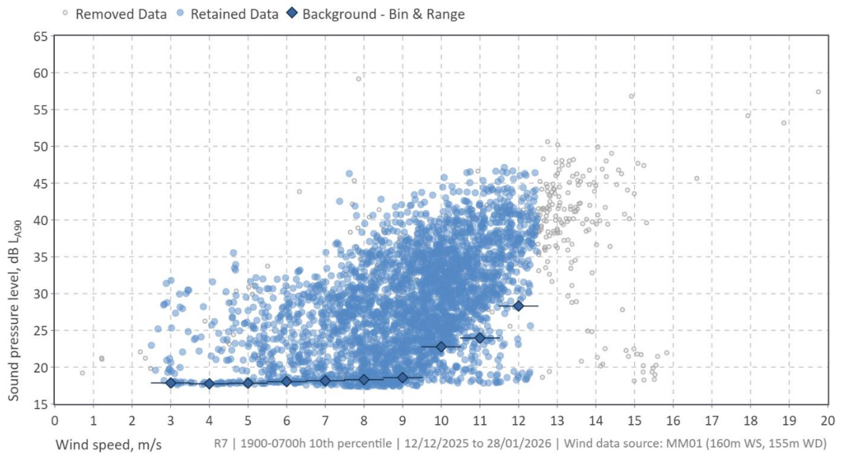
Figure 9: Location R7 derived background noise levels – 1900–0700 hrs (DWER 10 th percentile analysis)
