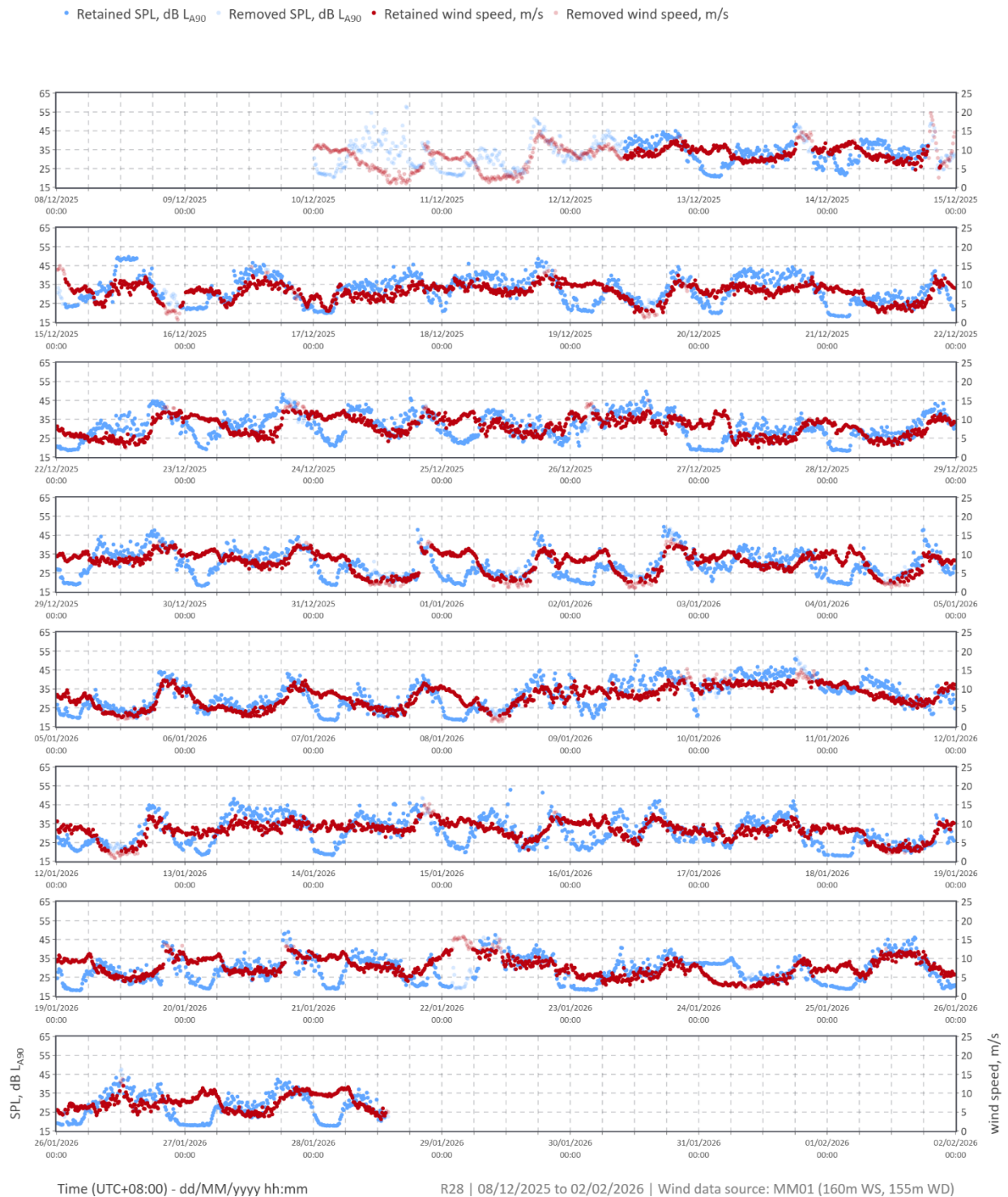
Figure 27: Location R28 background noise level and wind speed time history
