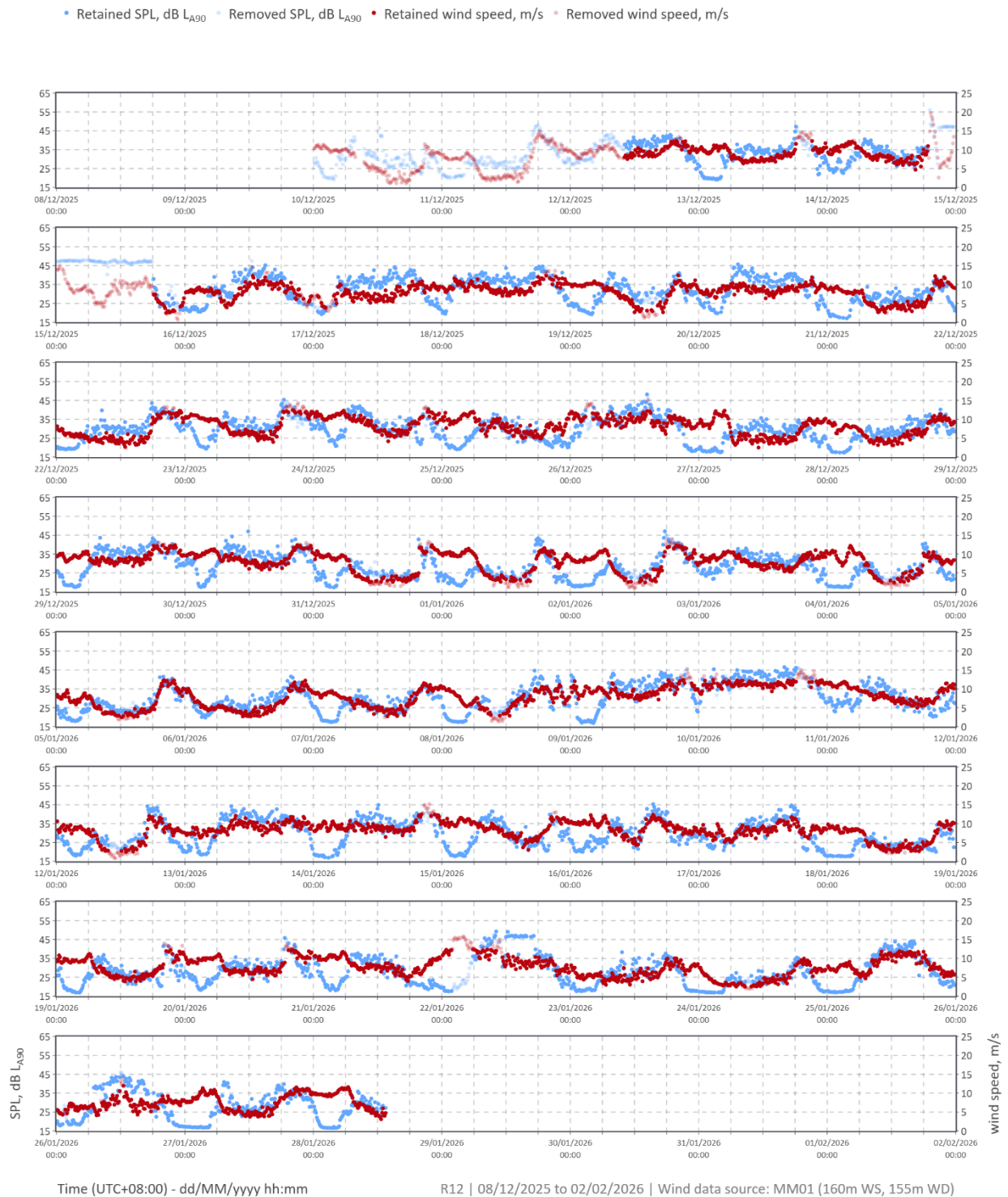
Figure 19: Location R12 background noise level and wind speed time history
