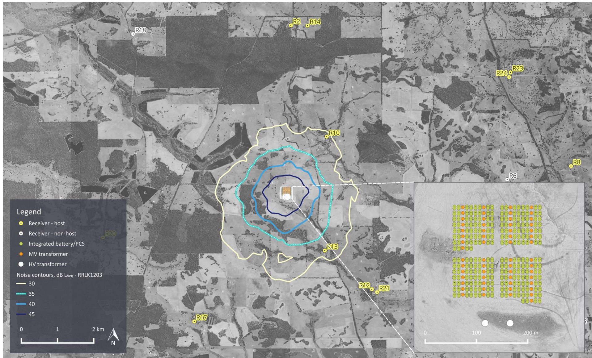
Figure 3: BESS site layout and predicted noise contours
