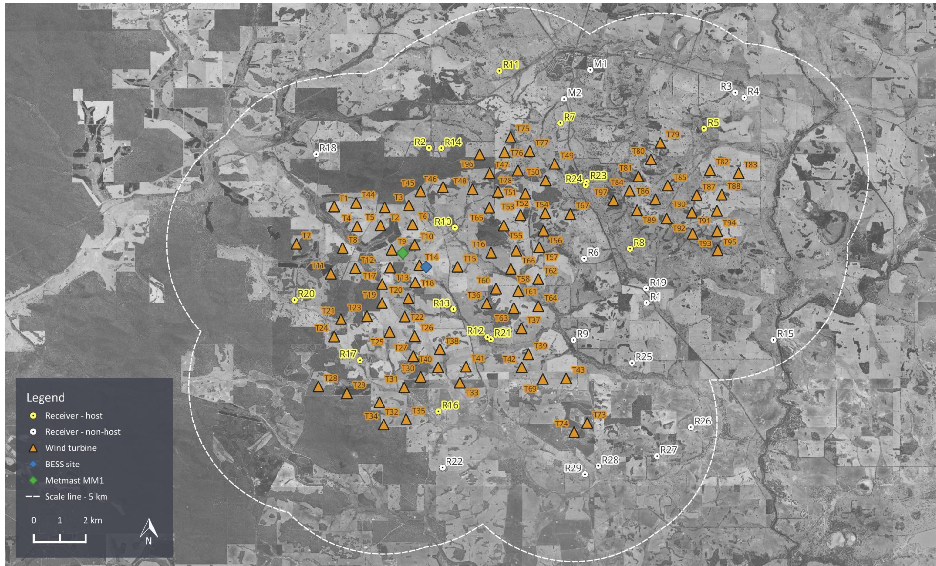
Figure 1: Project layout (layout 13072026WTGLayout)
