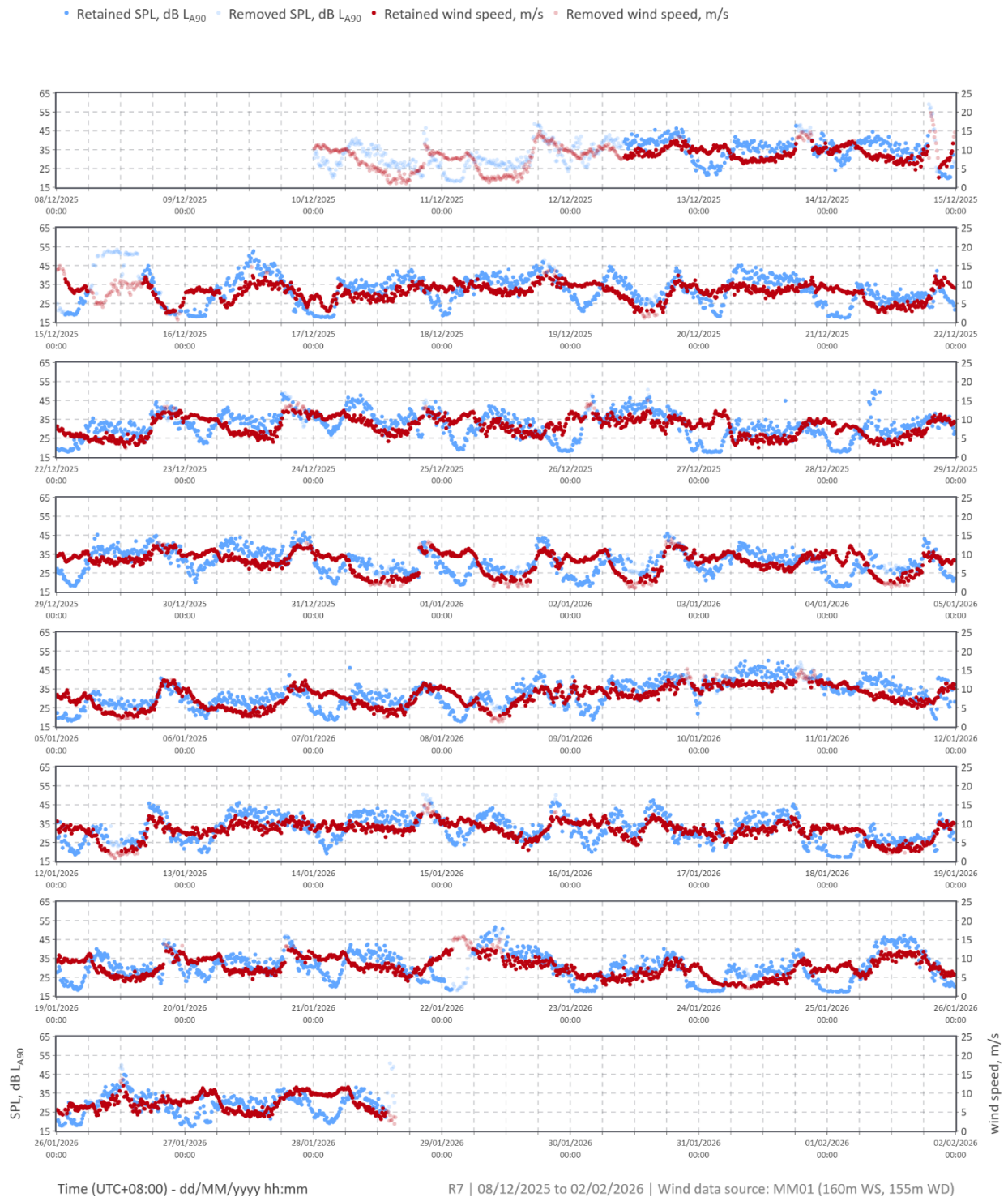
Figure 7: Location R7 background noise level and wind speed time history
