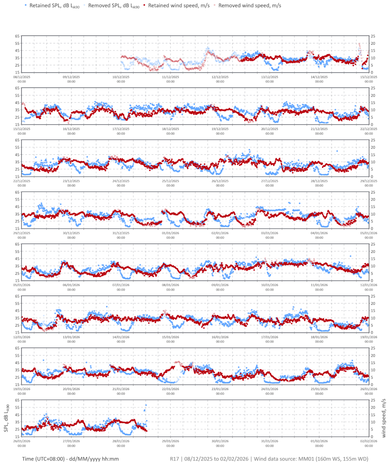
Figure 23: Location R17 background noise level and wind speed time history
