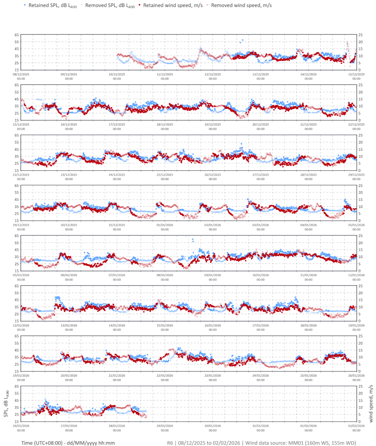
Figure 3: Location R6 background noise level and wind speed time history
