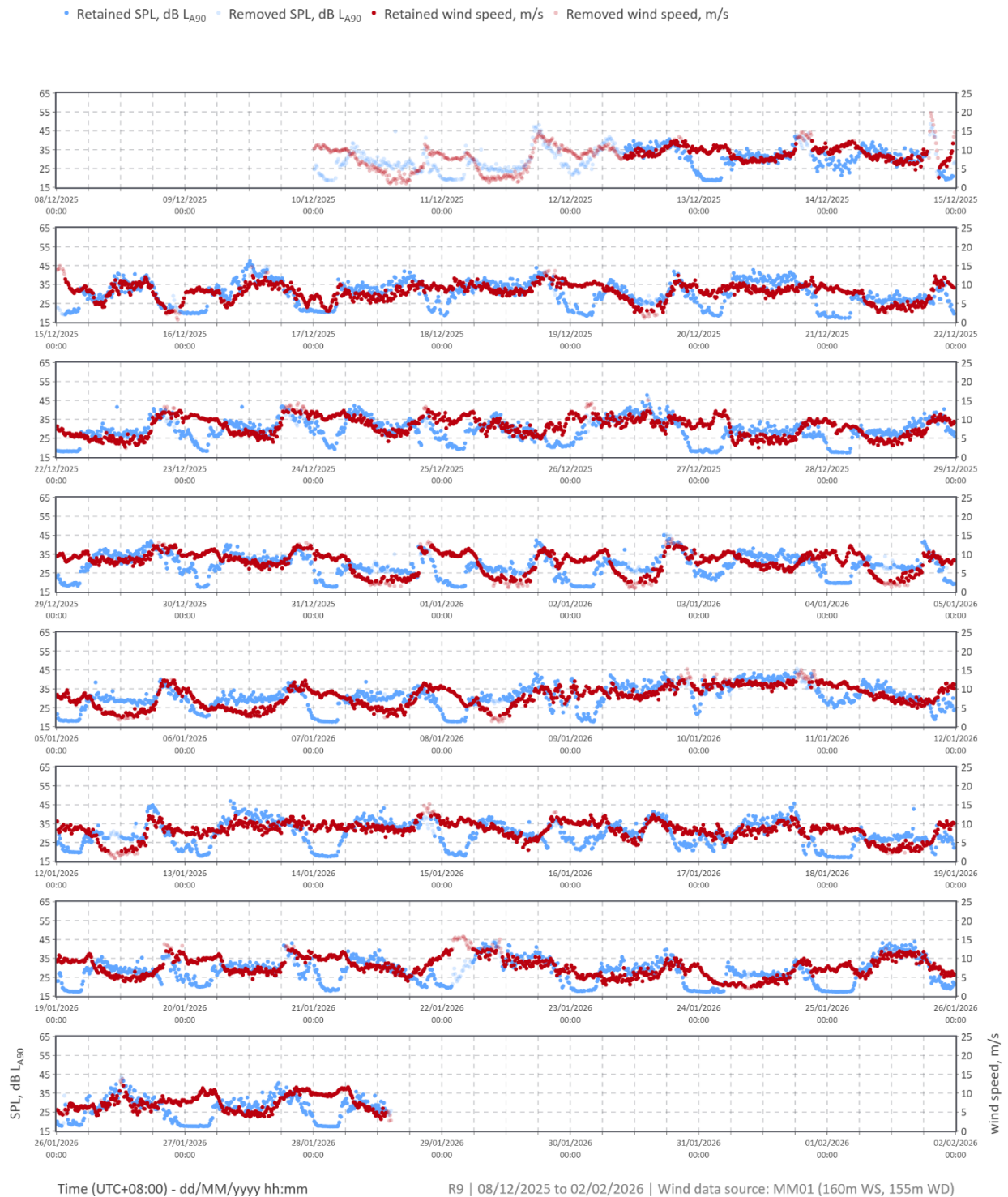
Figure 11: Location R9 background noise level and wind speed time history
