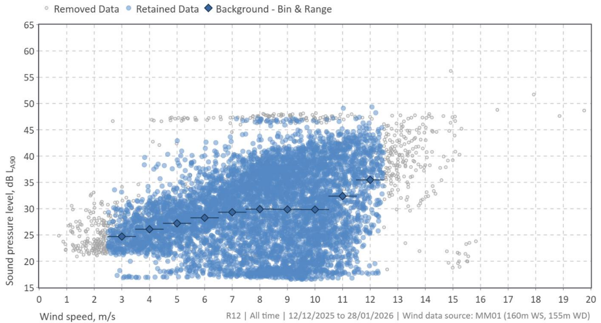
Figure 21: Location R12 derived background noise levels – 1900–0700 hrs (DWER 10 th percentile analysis)
