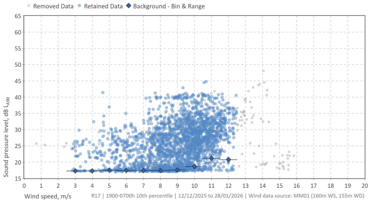
Figure 25: Location R17 derived background noise levels – 1900–0700 hrs (DWER 10 th percentile analysis)
