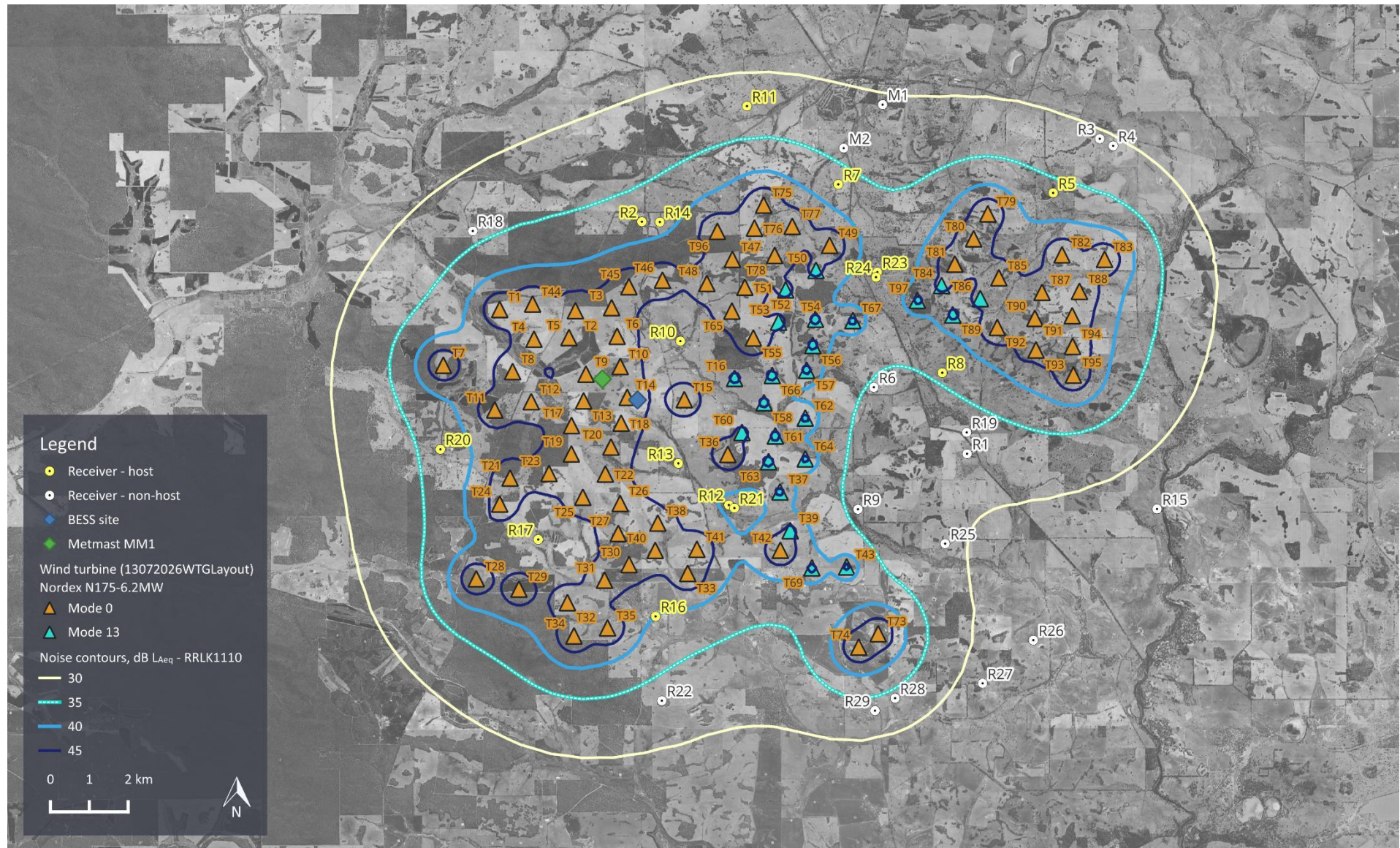
Figure 2: Predicted noise contours (layout 13072026WTGLayout, curtailed operation at 9 m/s hub height wind speed)
