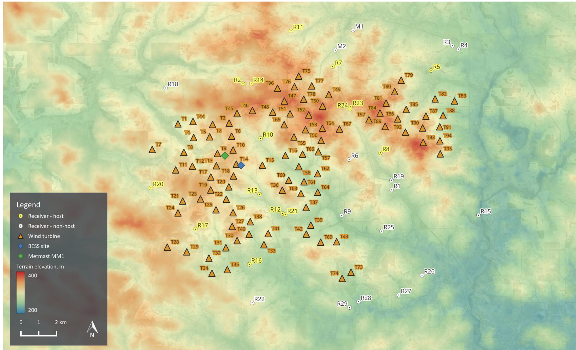
Figure 9: Site topography (layout 13072026WTGLayout)
